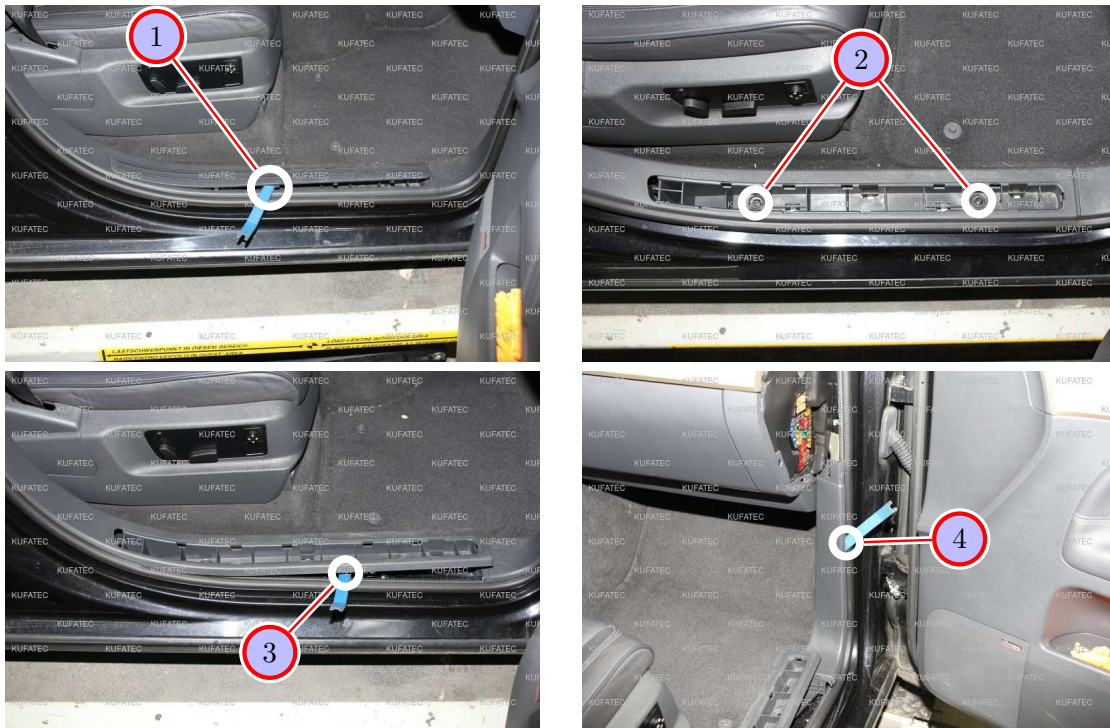
Figure 10: Removal cover parts passenger's side
