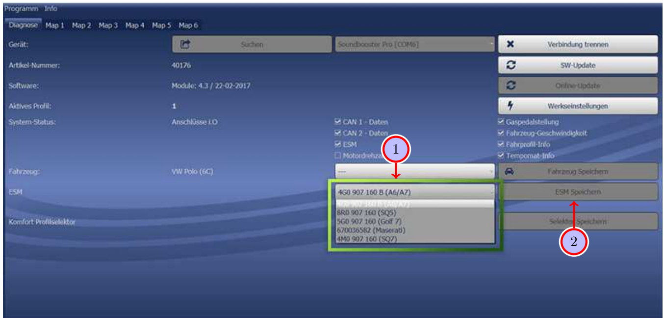
Figure 17: Software
