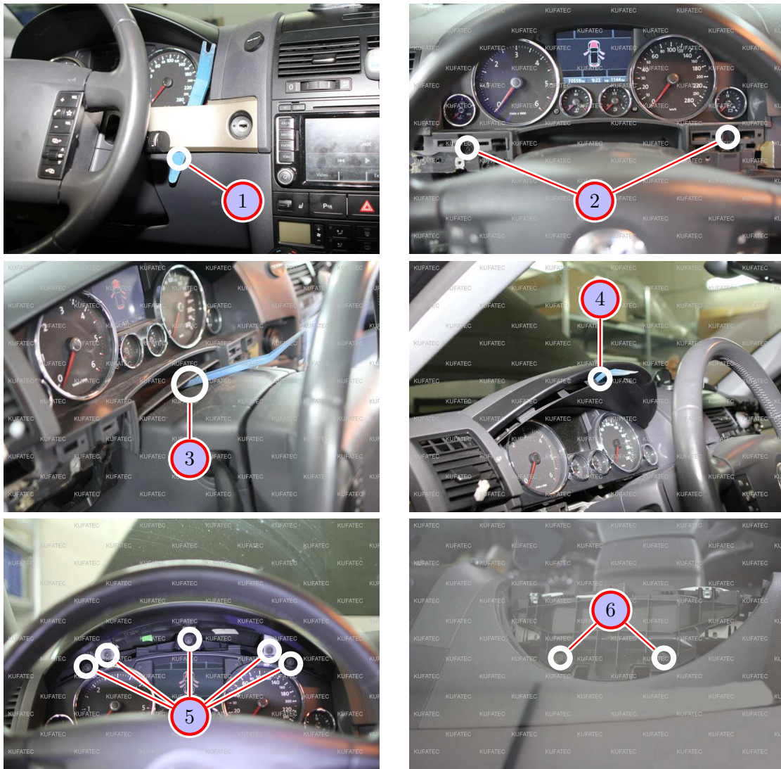
Figure 7: Removal tachometer
